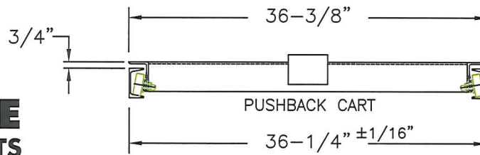
STANDARD SECTION OF 2 DEEP PUSHBACK SYSTEM
