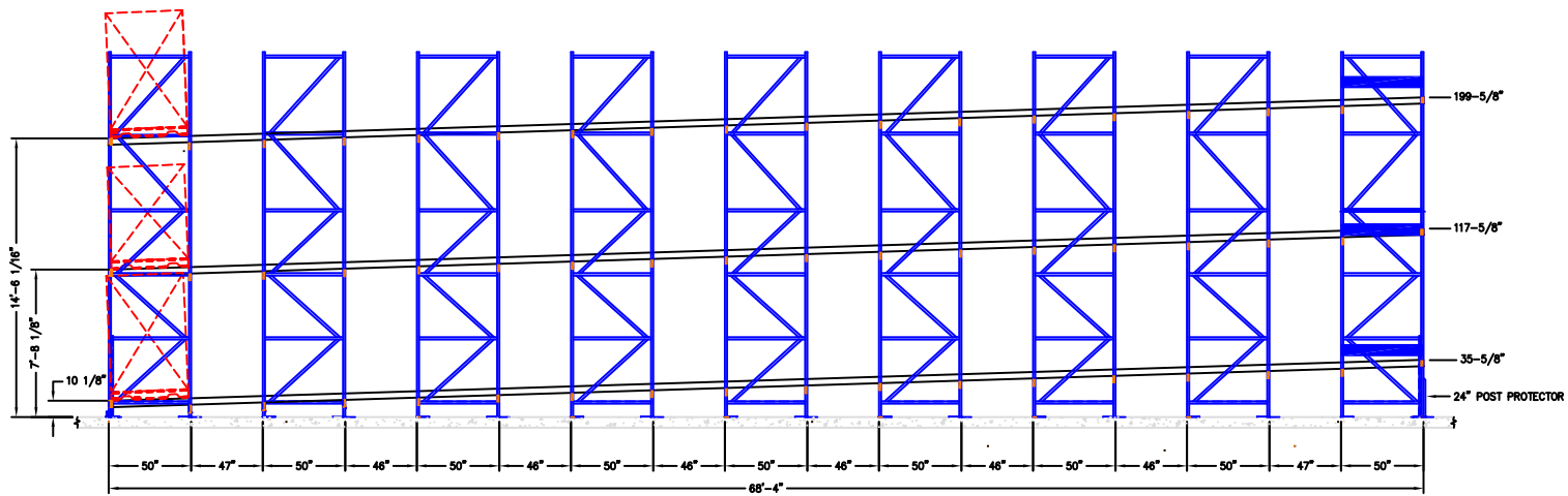
PALLET FLOW RACK SIDE ELEVATION 3/8" PITCH
