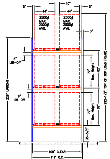
PALLET FLOW RACK REAR ELEVATION
